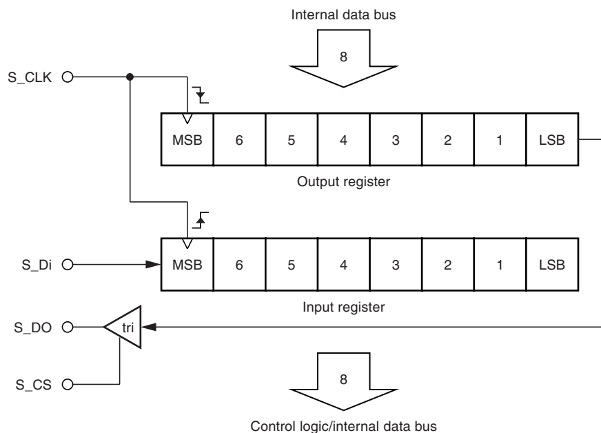
Figure 3-6. SPI Structure
