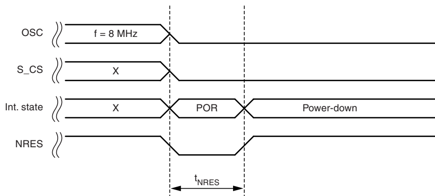
Figure 3-3. External Reset
