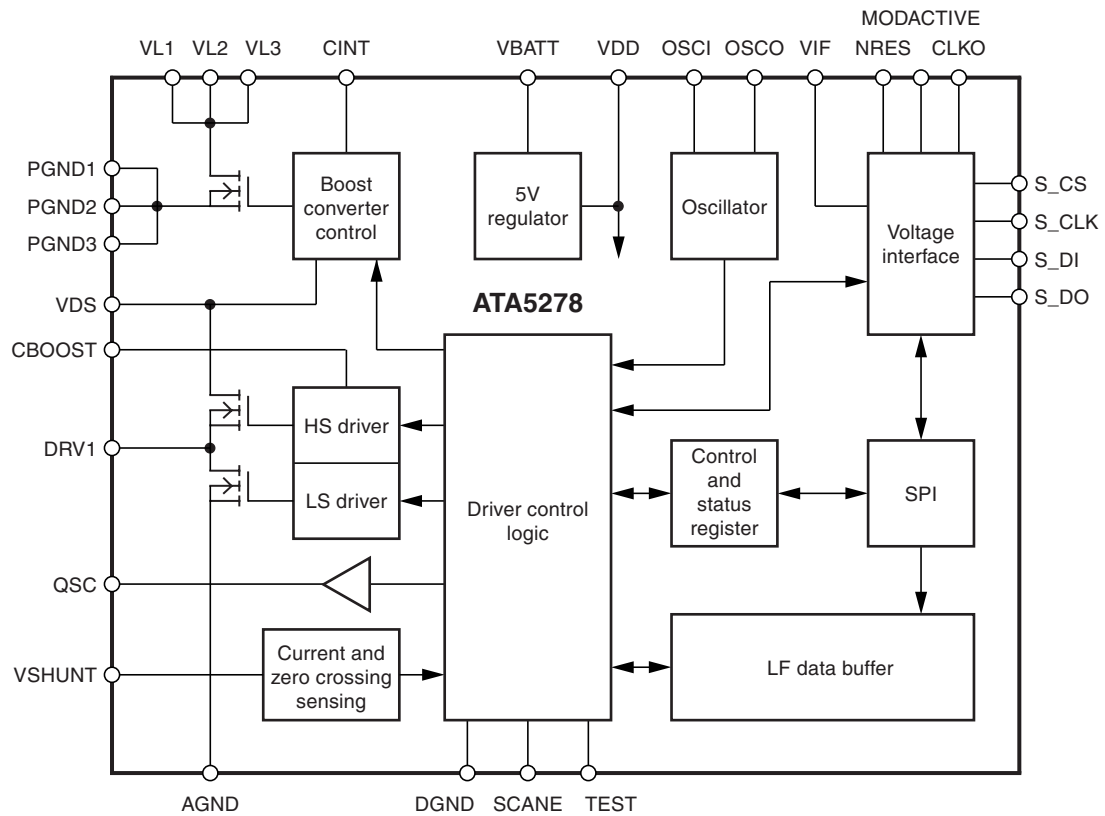
Figure 1-1. Block Diagram
